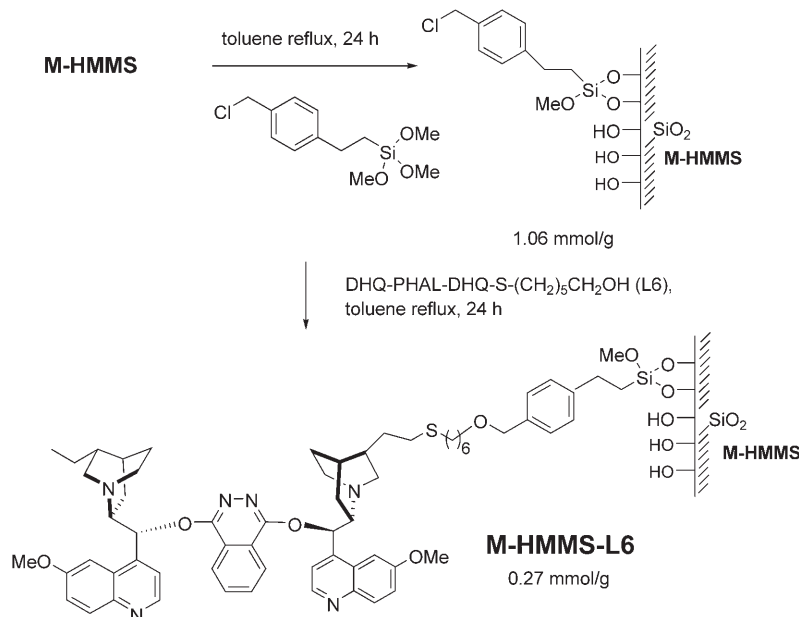
Scheme 1. Immobilization of chiral ligand L6 on M-HMMS.
