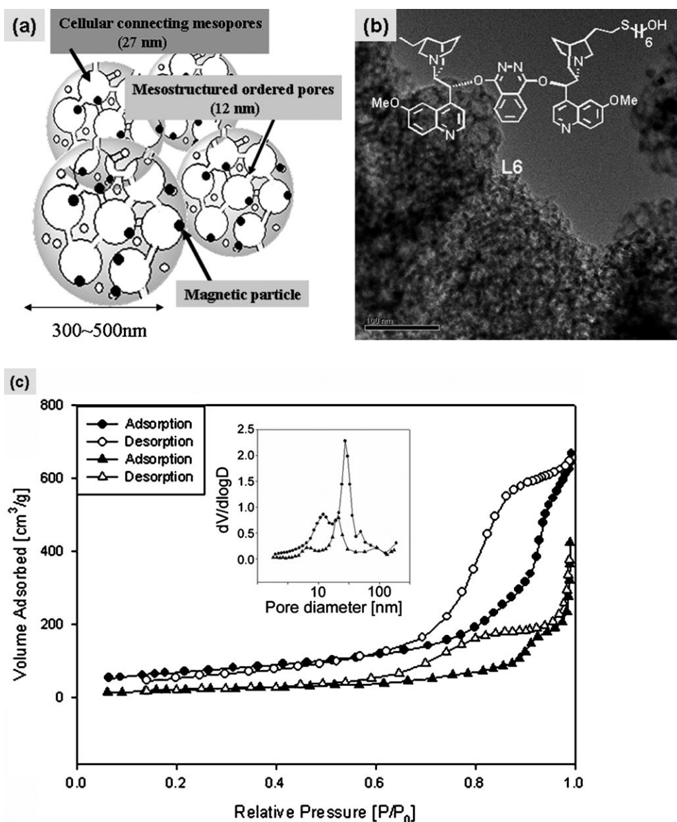
Figure 2. (a) Pictorial representation of M-HMMS, (b) structure of the modified ligand L6 and the TEM image of M-HMMS-L6, (c) N 2 adsorption-desorption isotherm of magnetic M-MMS (●) and M-MMS-L6 (▲) including calculated pore diameter by the BJH method.
