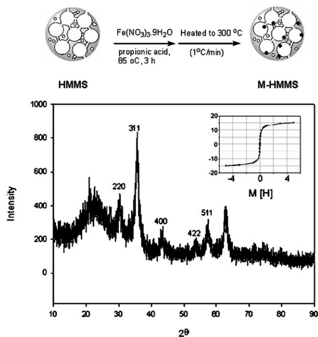
Figure 1. Preparation of iron-nanoparticle encapsulated mesostructured material and physical data: wide-angle XRD pattern of M-HMMS and magnetization curve of M-HMMS.
