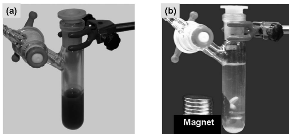
Figure 3. (a) AD reaction mixture containing M-HMMS-L6, and (b) M-HMMS-L6 collected using an external magnet after the reaction.
